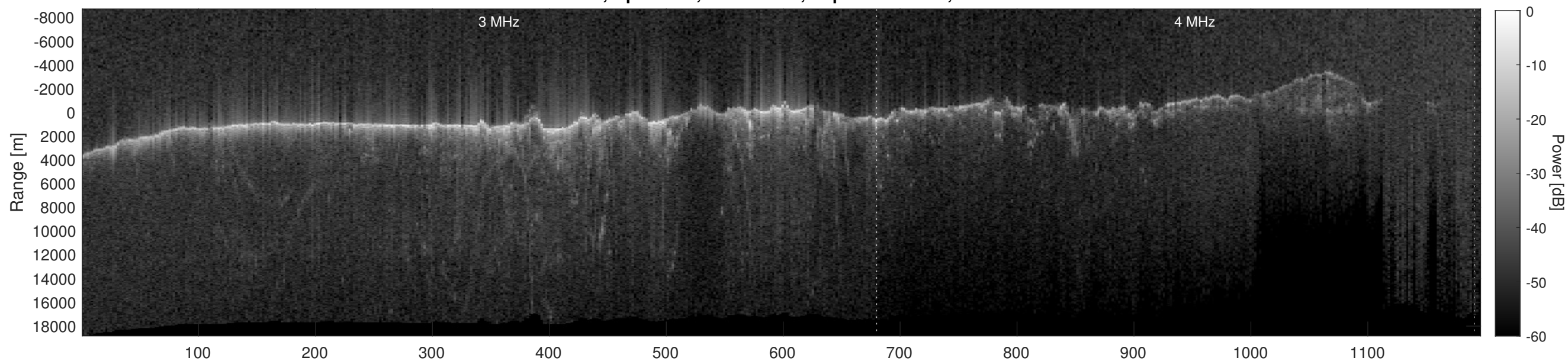
Orbit 6877, Depth-Corrected Cluttergram
