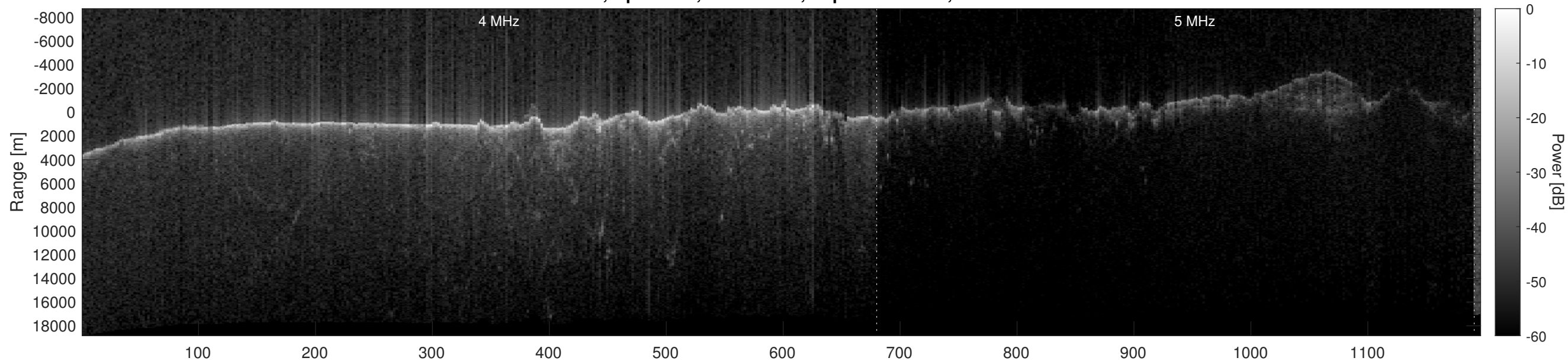
Orbit 6877, Optimized, No Window, Depth-Corrected, Channel 2
