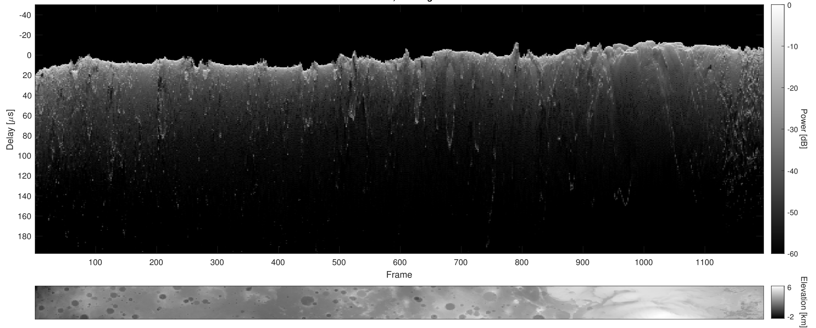
Orbit 6878, Cluttergram
