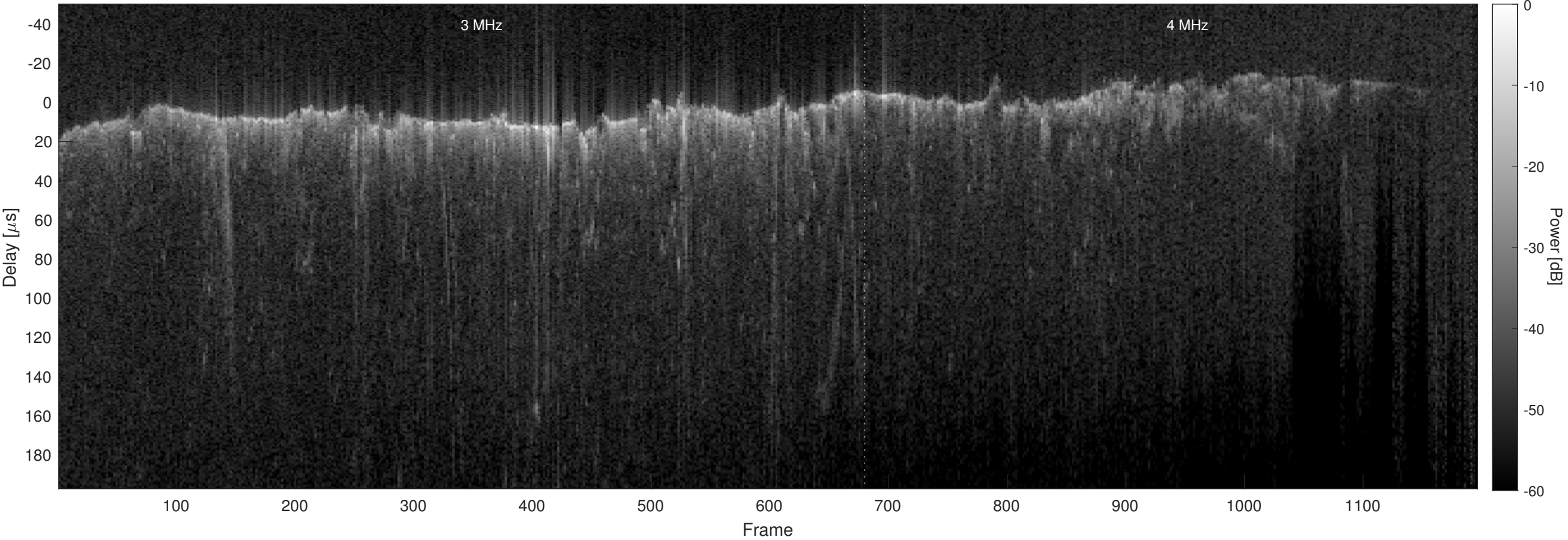
Orbit 6878, Optimized, No Window, Channel 2
