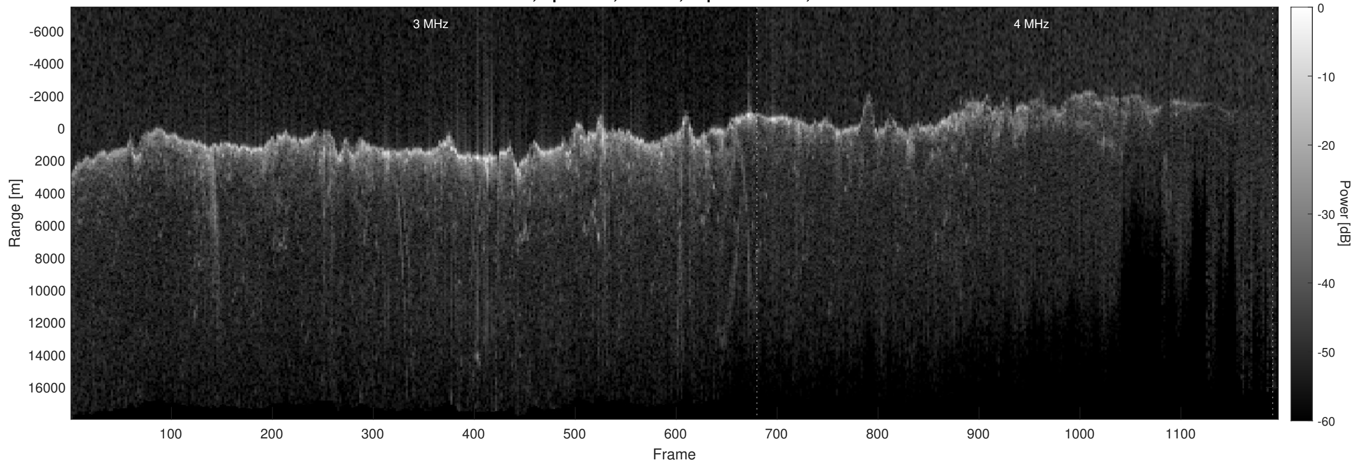
Orbit 6878, Optimized, Window, Depth-Corrected, Channel 2
