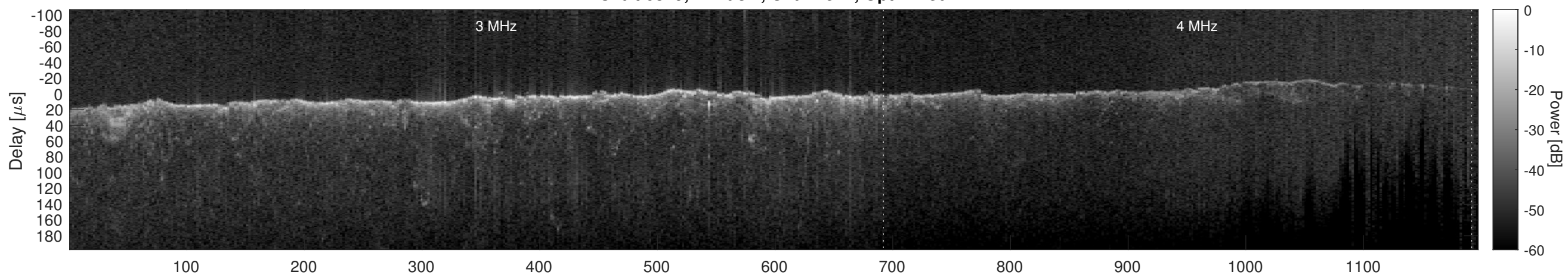
Orbit 6879, Cluttergram
