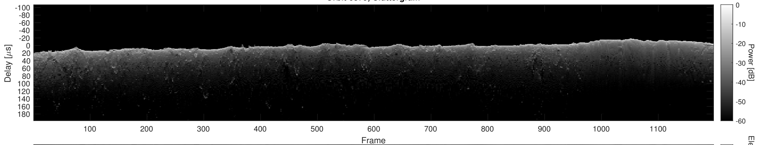
Orbit 6879, Cluttergram
