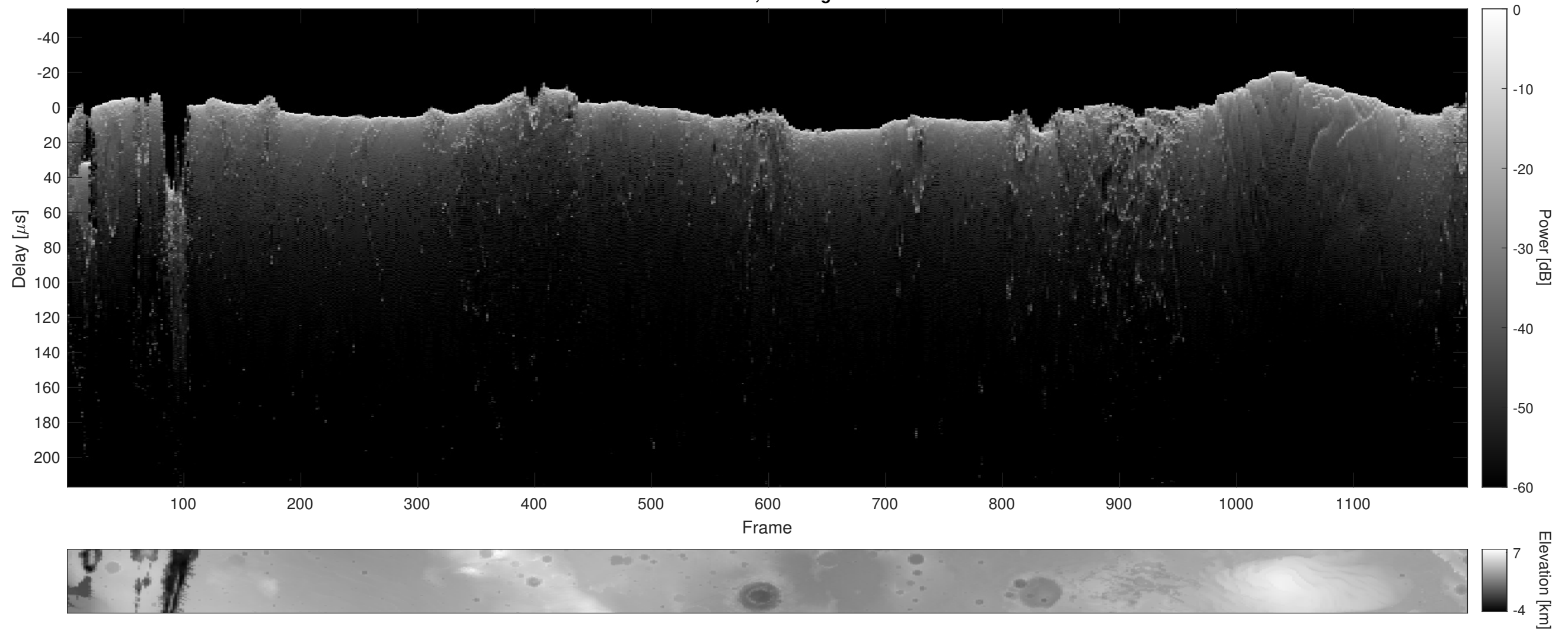
Orbit 6880, Cluttergram
