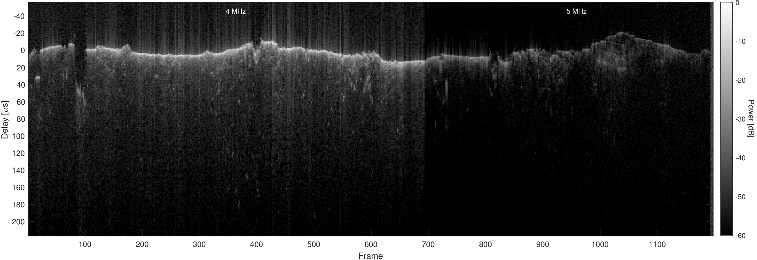
Orbit 6880, Optimized, No Window, Channel 2
