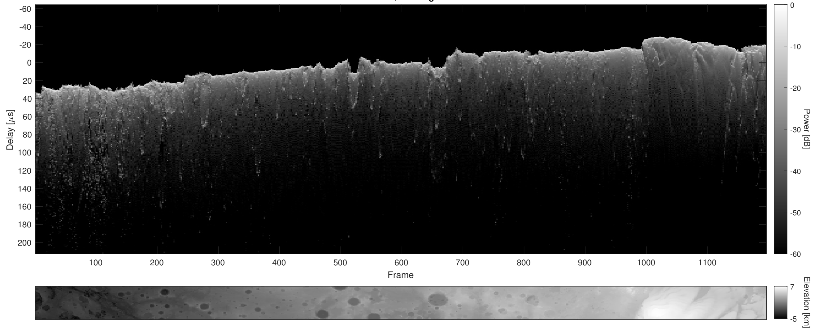
Orbit 6883, Cluttergram
