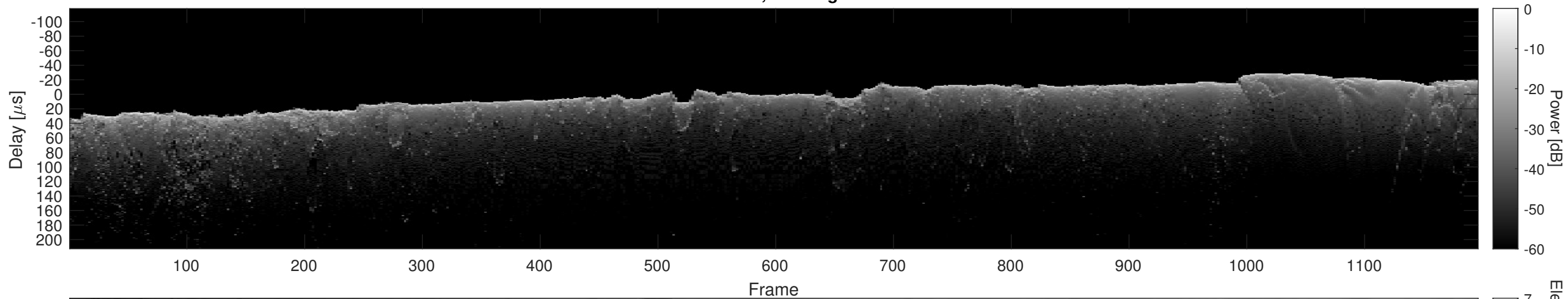
Orbit 6883, Cluttergram
