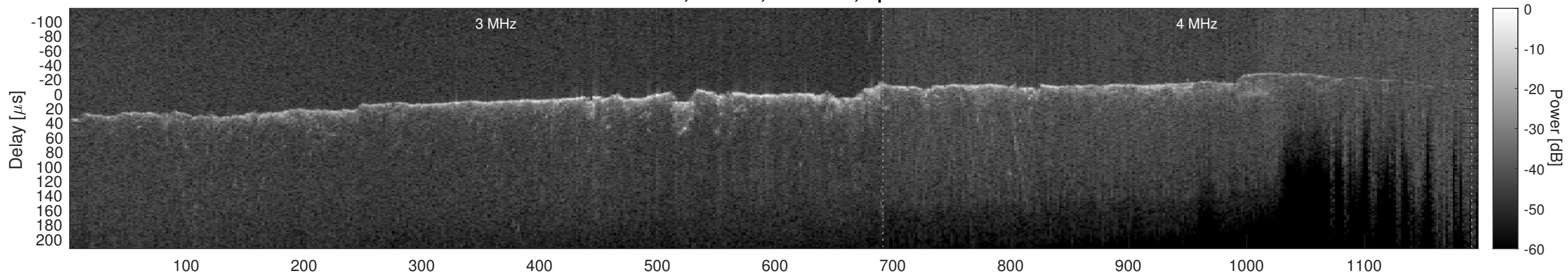
Orbit 6883, Cluttergram
