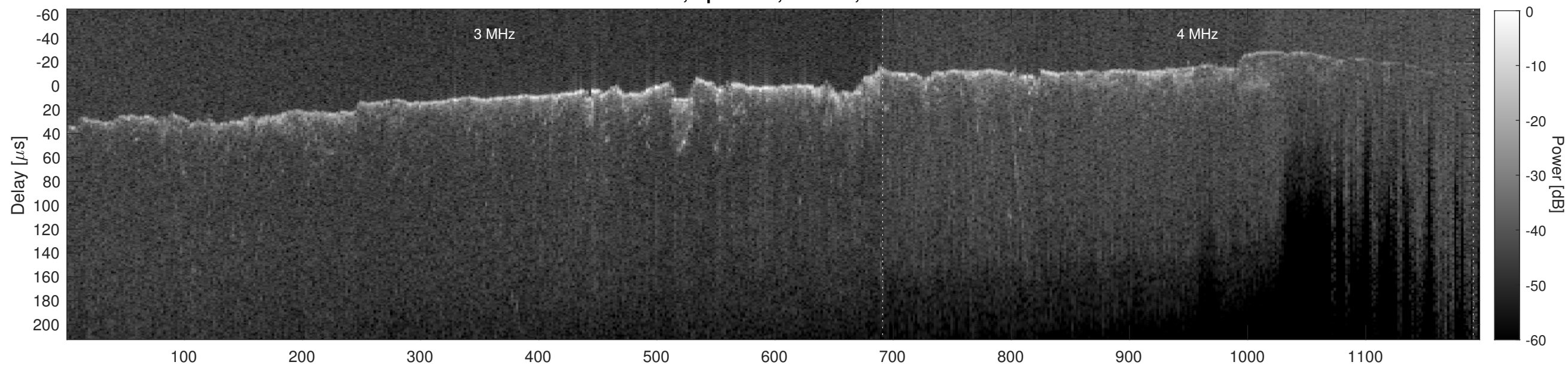
Orbit 6883, Cluttergram
