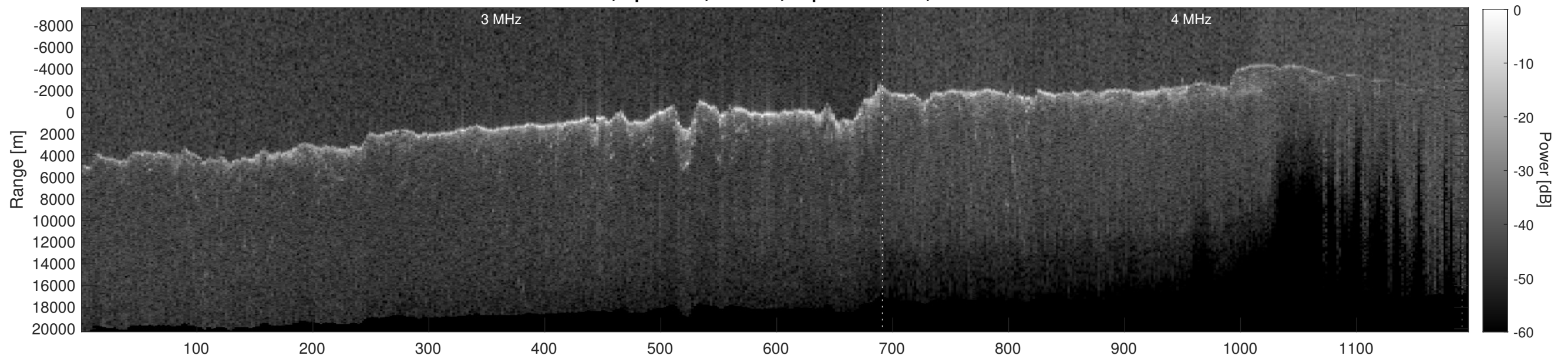
Orbit 6883, Depth-Corrected Cluttergram
