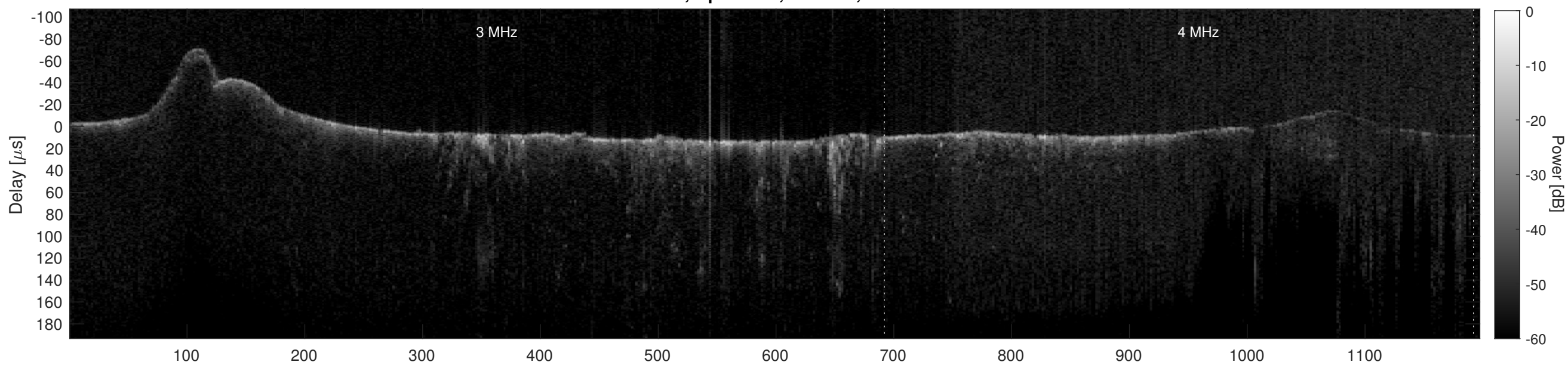
Orbit 6884, Cluttergram
