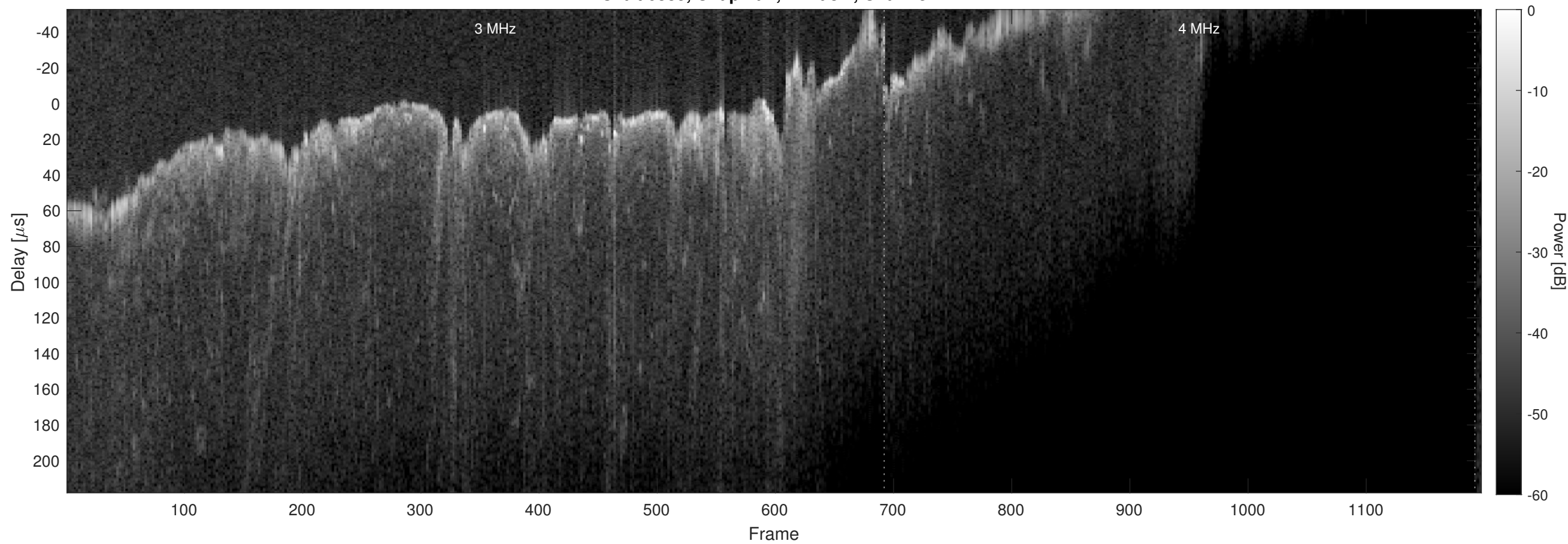
Orbit 6885, Chapman, Window, Channel 2
