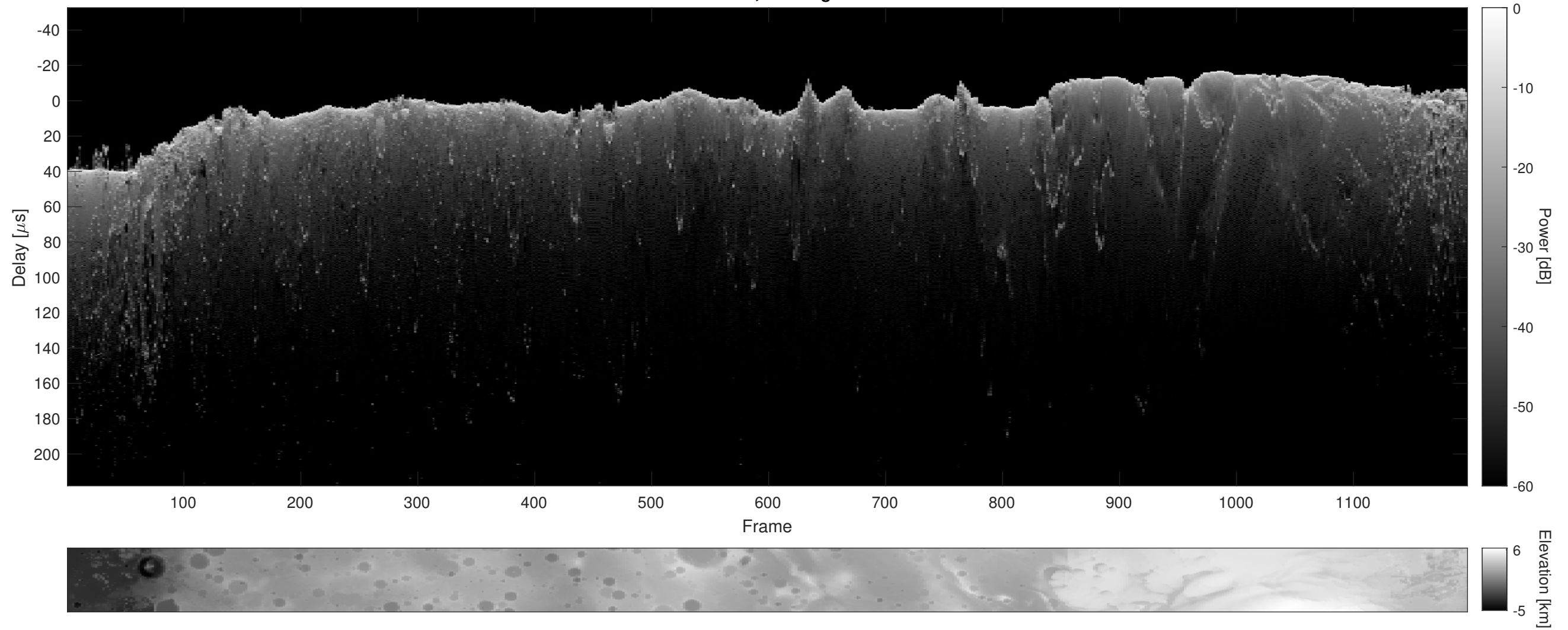
Orbit 6885, Cluttergram
