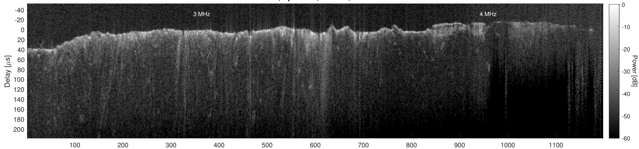
Orbit 6885, Cluttergram
