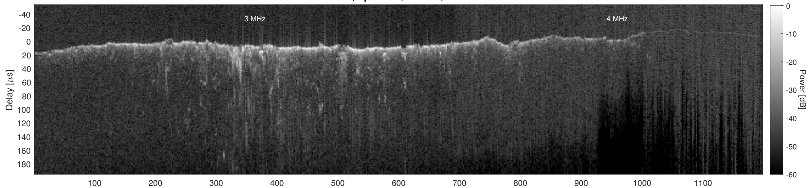
Orbit 6886, Cluttergram
