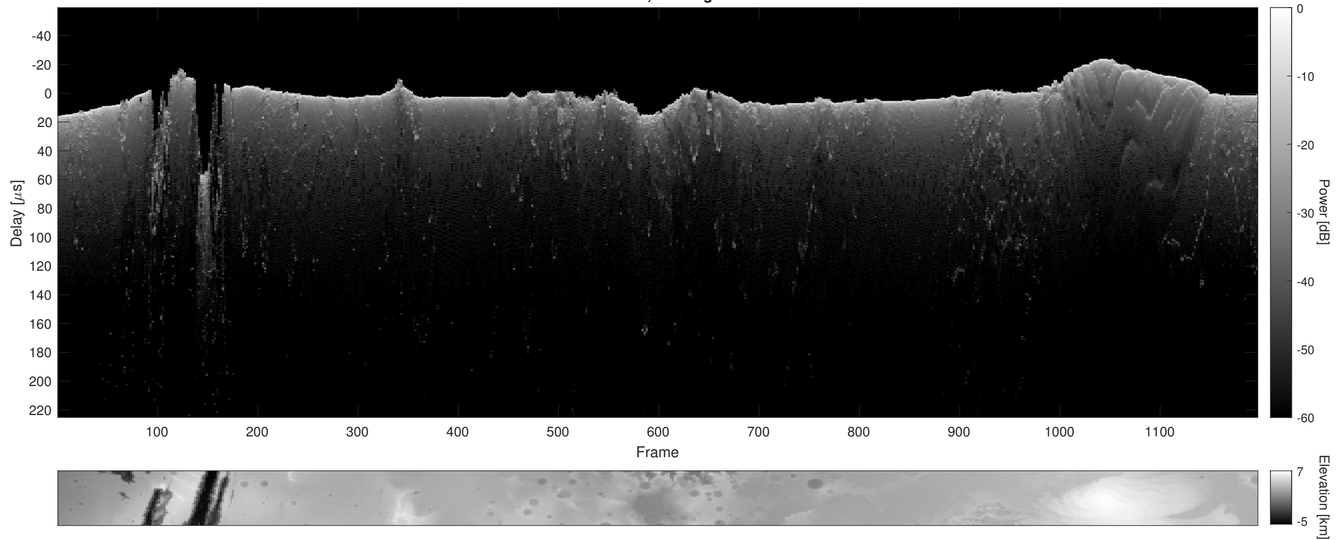
Orbit 6887, Cluttergram
