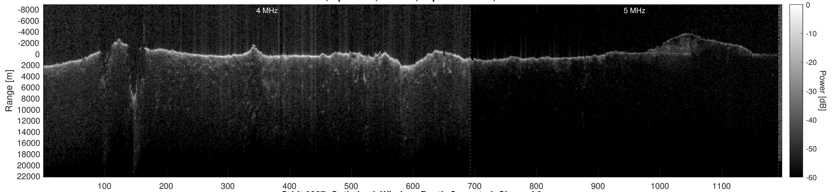
Orbit 6887, Optimized, Window, Depth-Corrected, Channel 2
