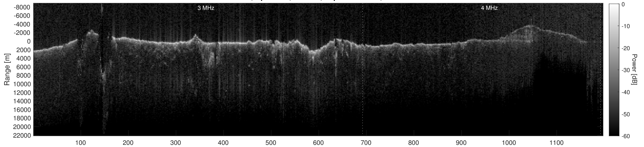
Orbit 6887, Depth-Corrected Cluttergram
