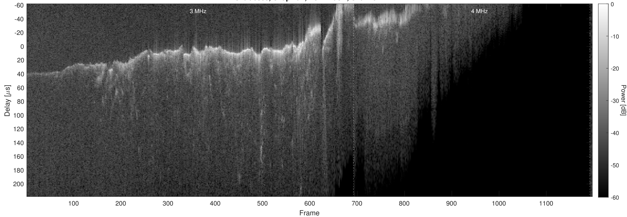
Orbit 6888, Chapman, No Window, Channel 2
