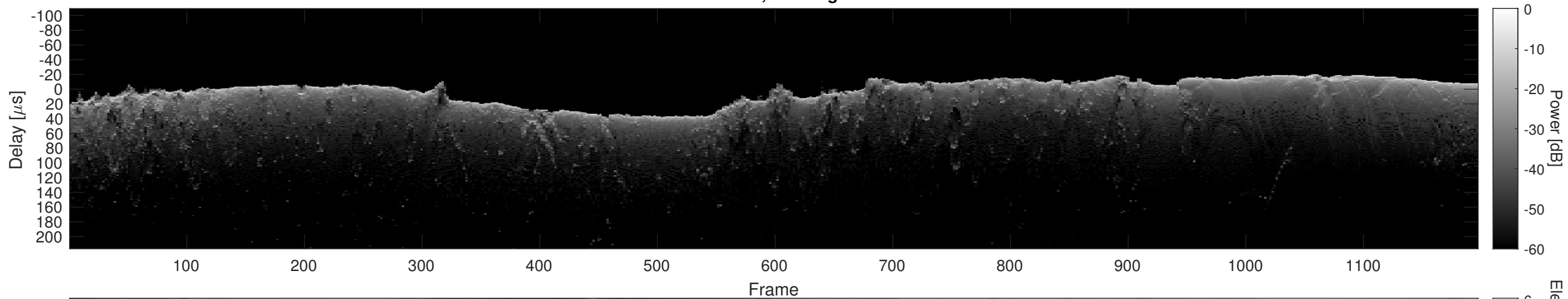
Orbit 6889, Cluttergram
