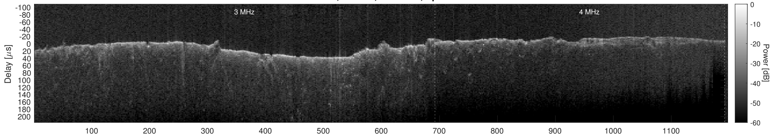
Orbit 6889, Cluttergram
