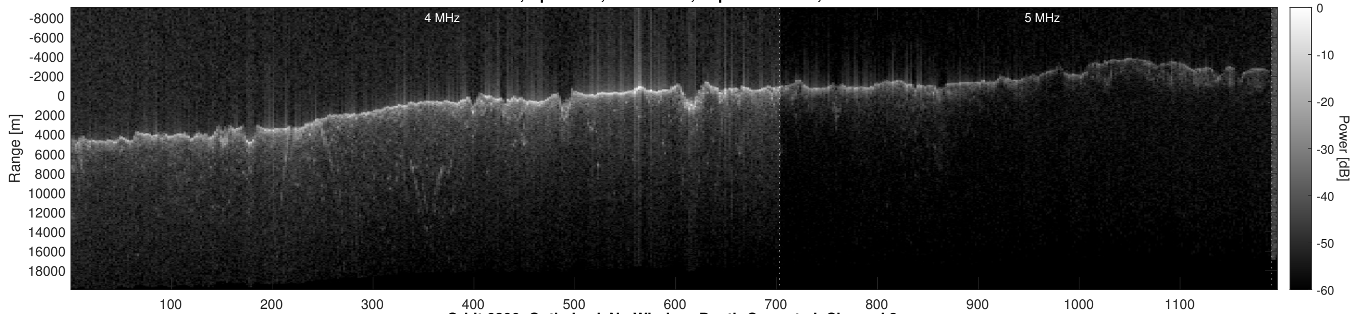
Orbit 6890, Optimized, No Window, Depth-Corrected, Channel 2
