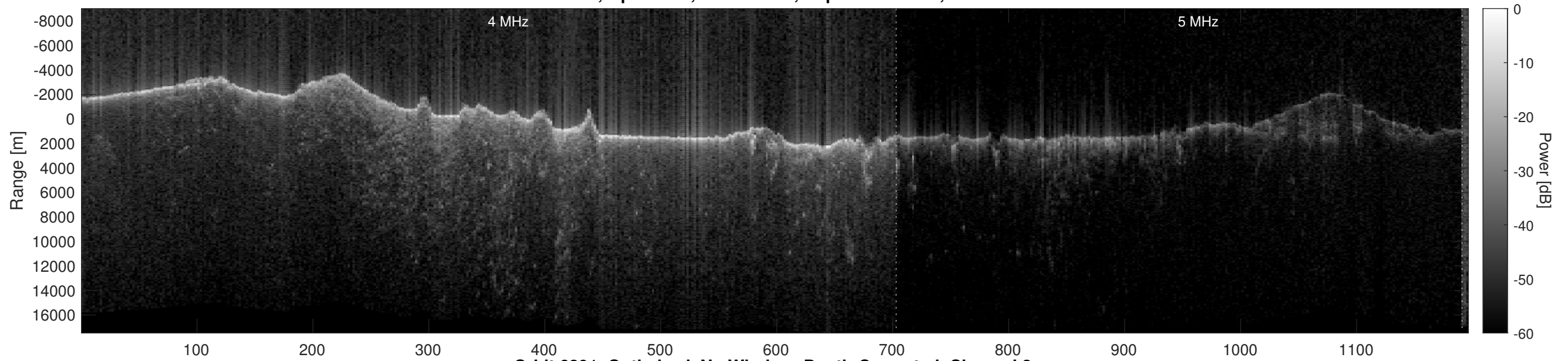
Orbit 6891, Optimized, No Window, Depth-Corrected, Channel 2
