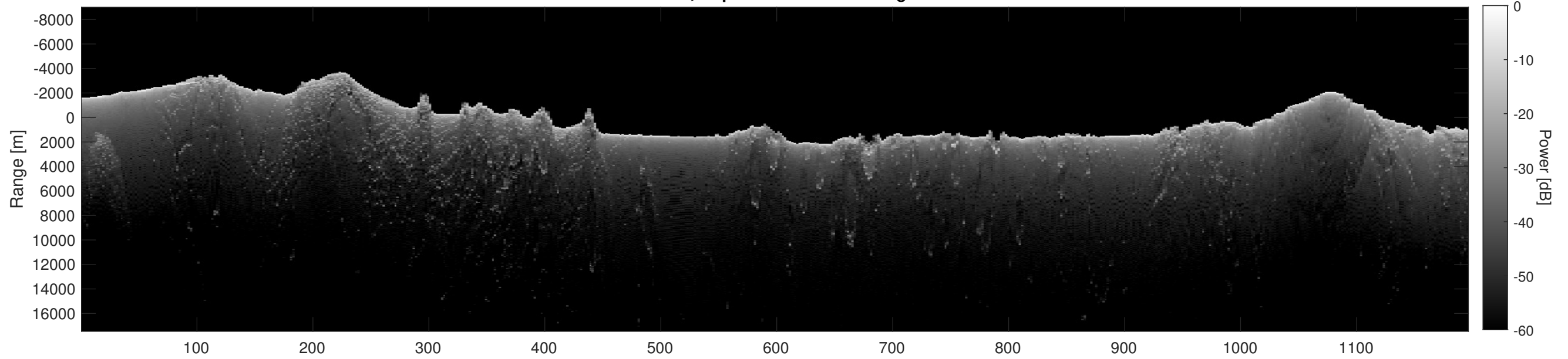
Orbit 6891, Depth-Corrected Cluttergram
