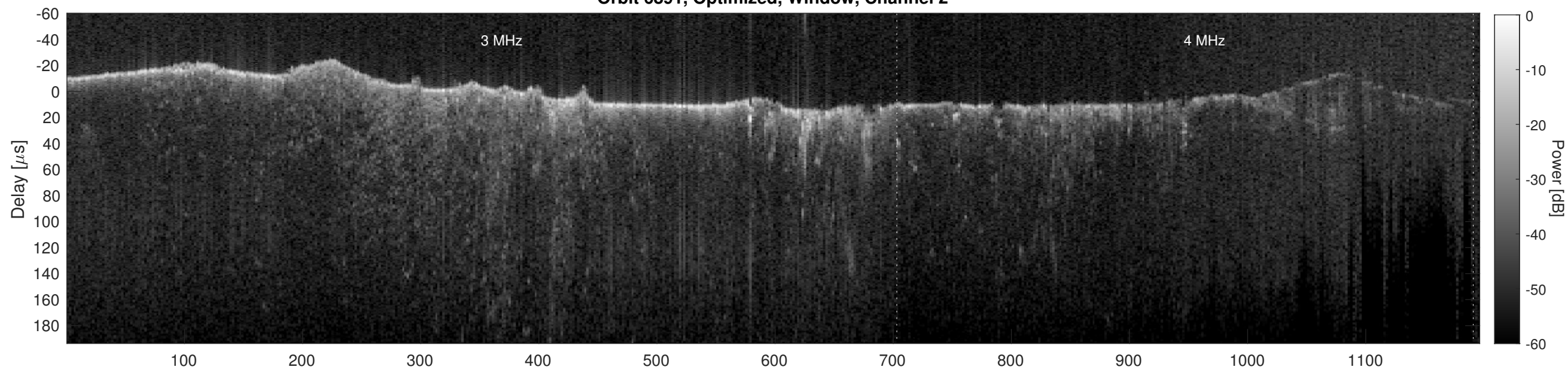
Orbit 6891, Cluttergram
