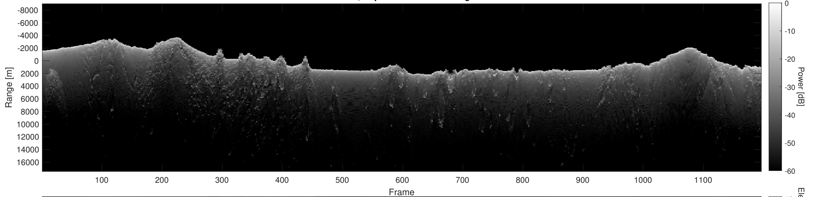
Orbit 6891, Depth-Corrected Cluttergram
