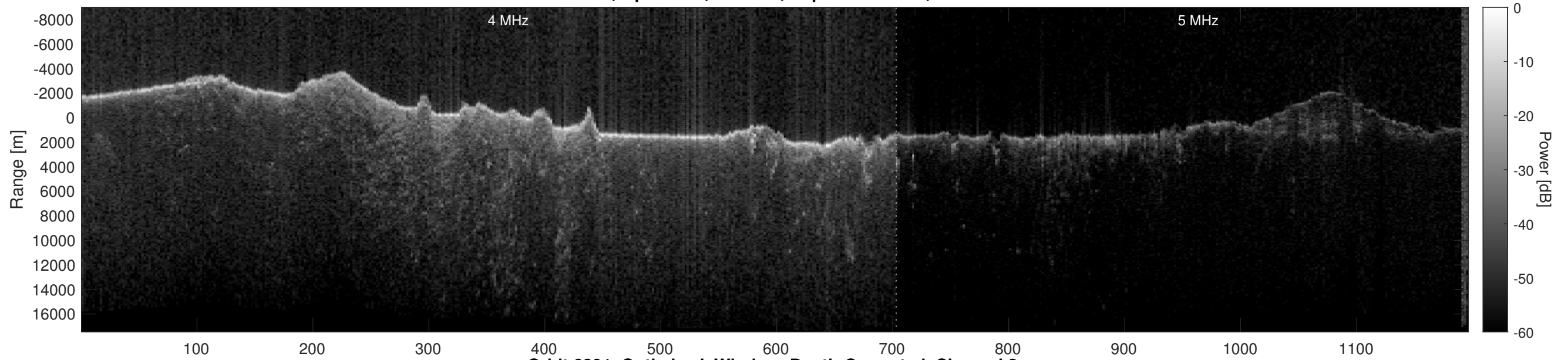
Orbit 6891, Optimized, Window, Depth-Corrected, Channel 2
