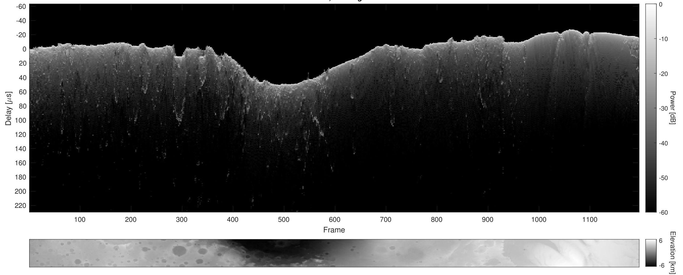
Orbit 6893, Cluttergram
