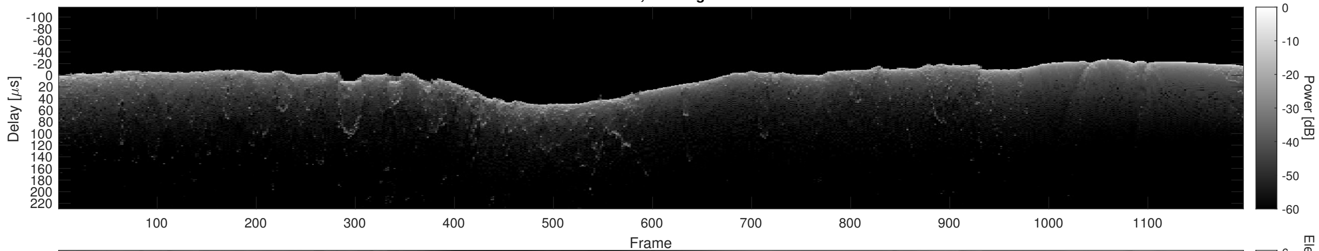
Orbit 6893, Cluttergram
