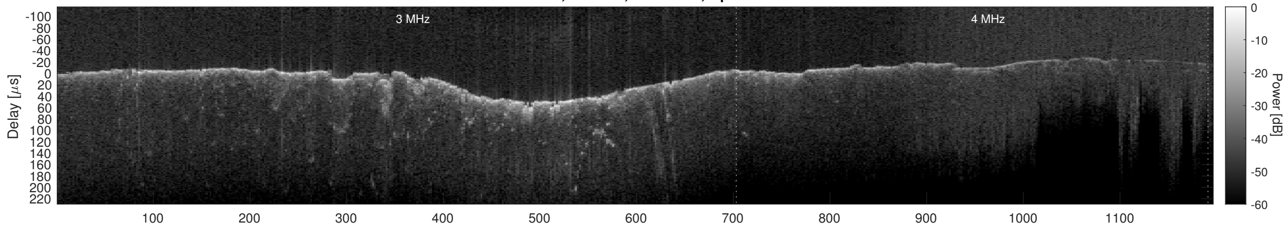
Orbit 6893, Cluttergram
