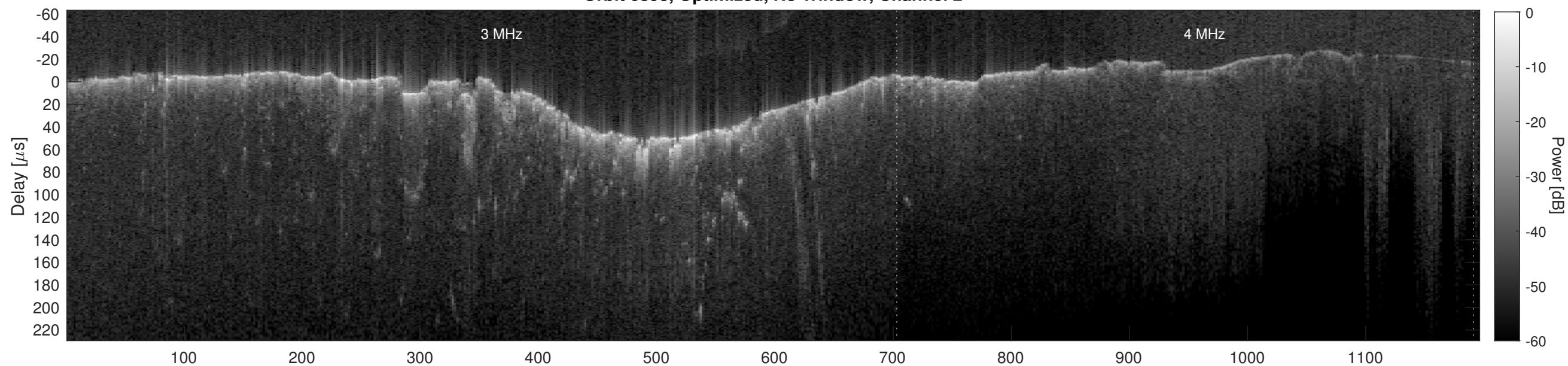
Orbit 6893, Cluttergram
