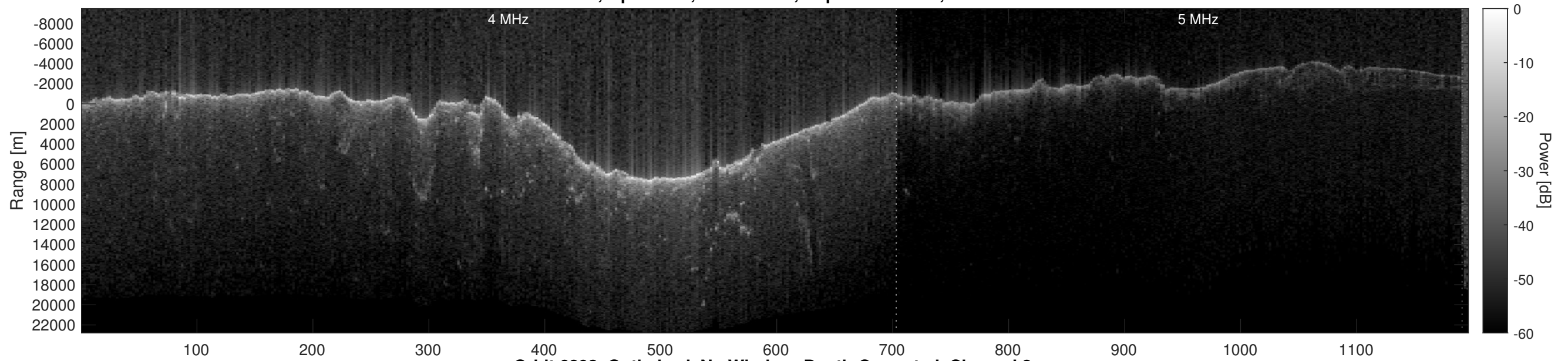
Orbit 6893, Optimized, No Window, Depth-Corrected, Channel 2
