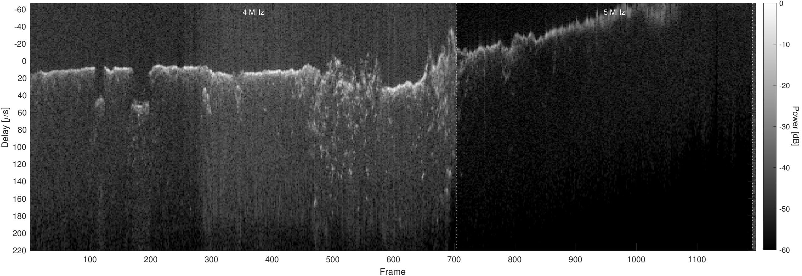
Orbit 6894, Chapman, Window, Channel 2
