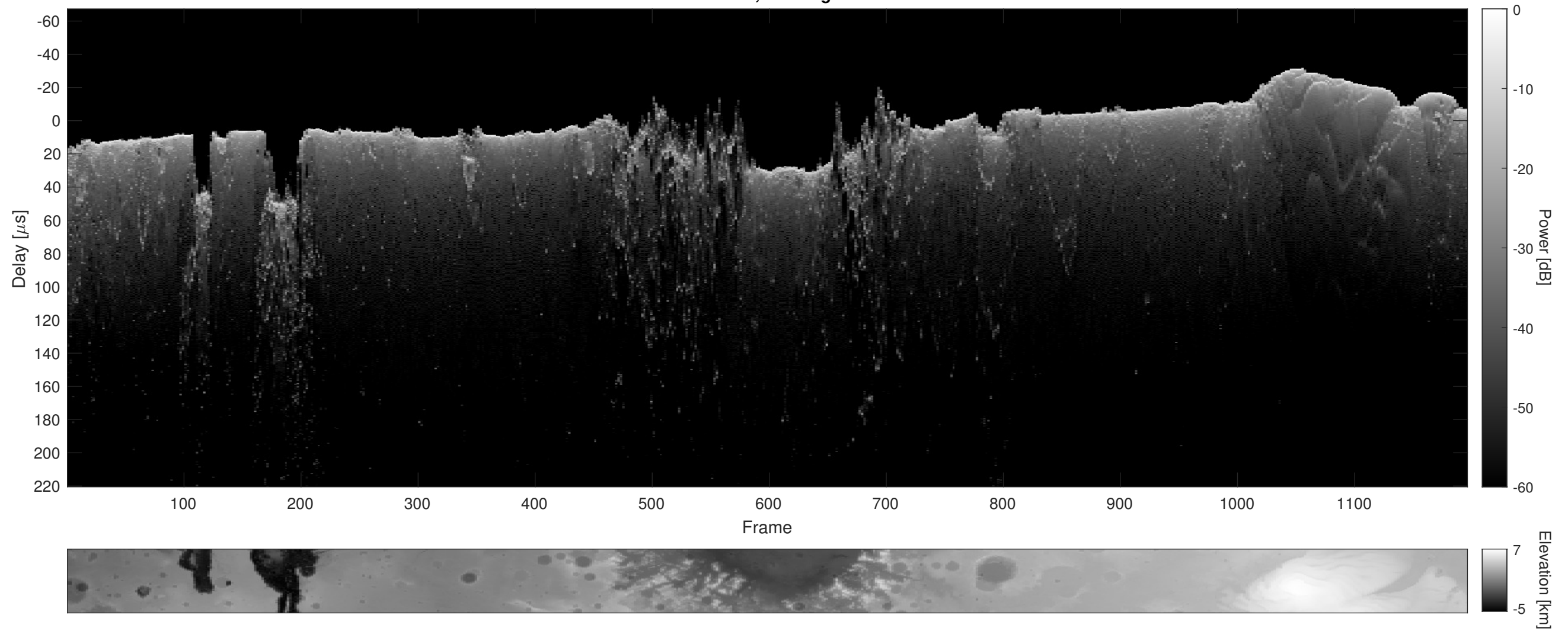
Orbit 6894, Cluttergram
