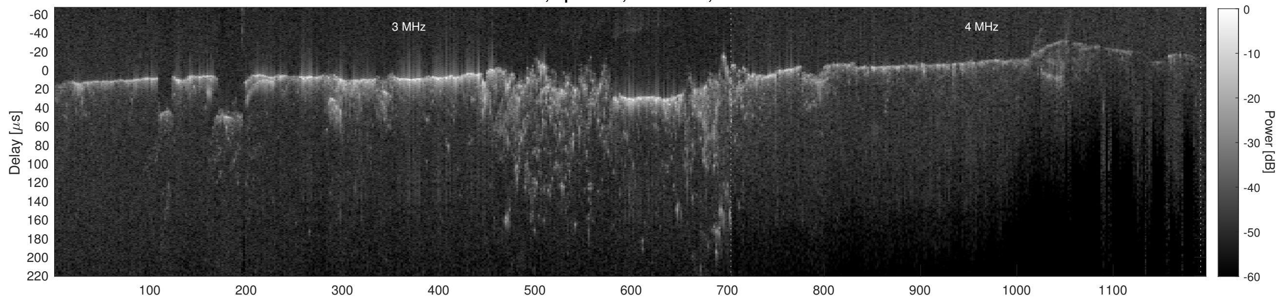
Orbit 6894, Cluttergram
