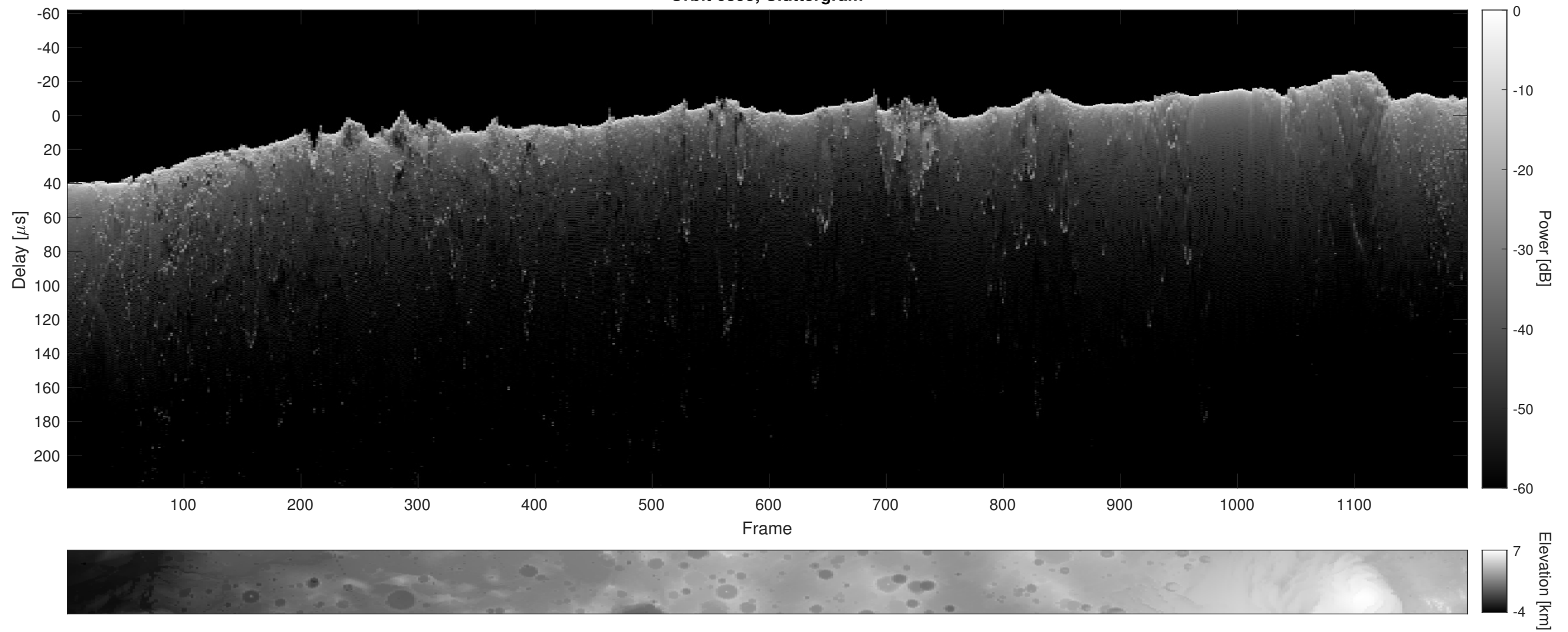
Orbit 6895, Cluttergram
