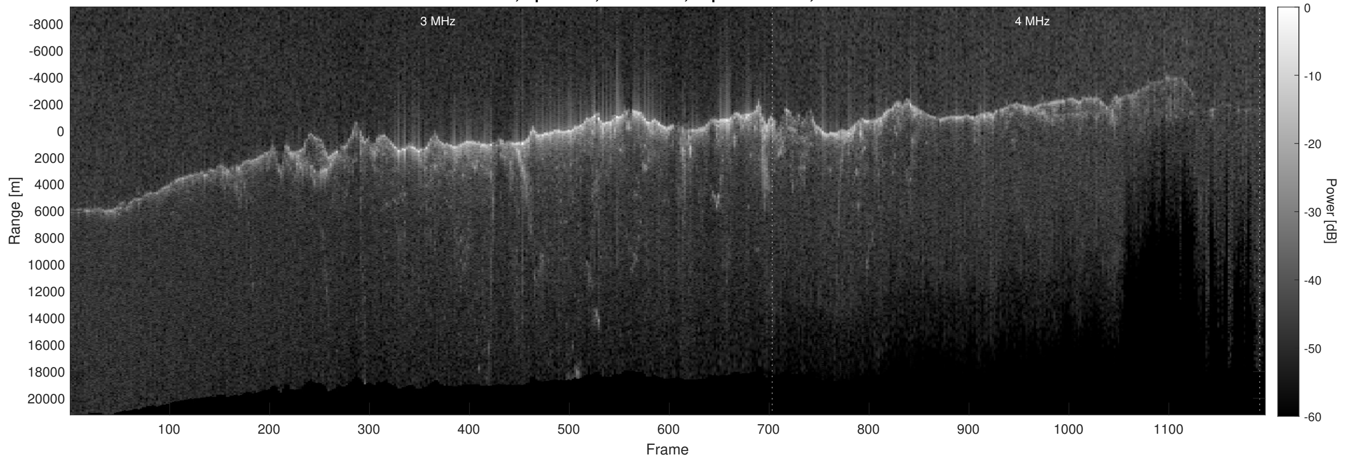
Orbit 6895, Optimized, No Window, Depth-Corrected, Channel 2
