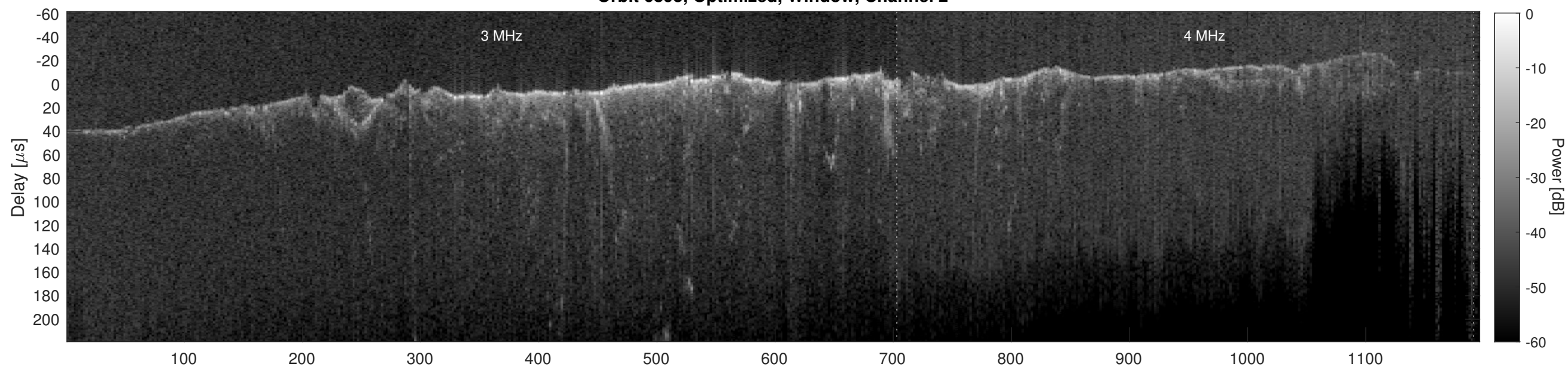
Orbit 6895, Cluttergram
