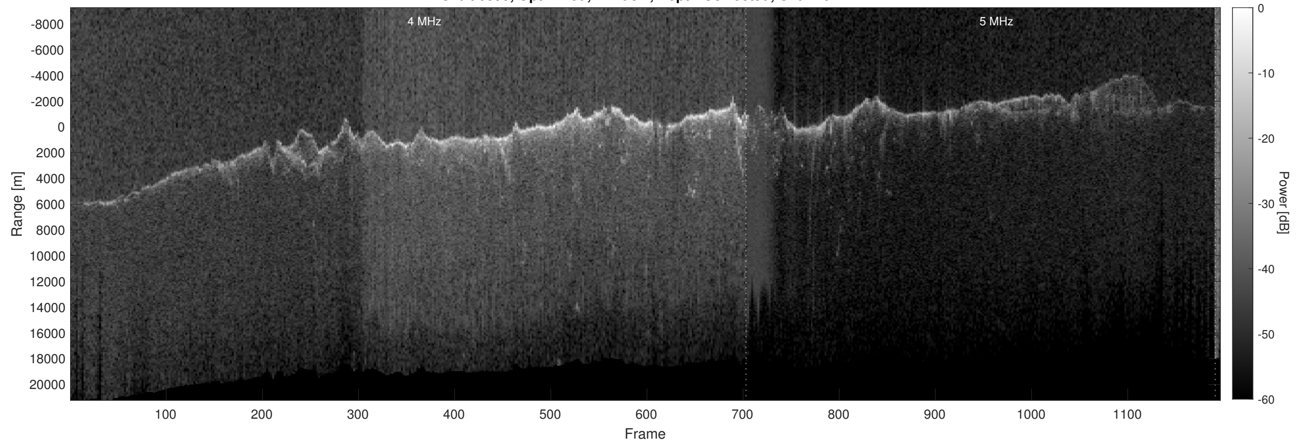
Orbit 6895, Optimized, Window, Depth-Corrected, Channel 2
