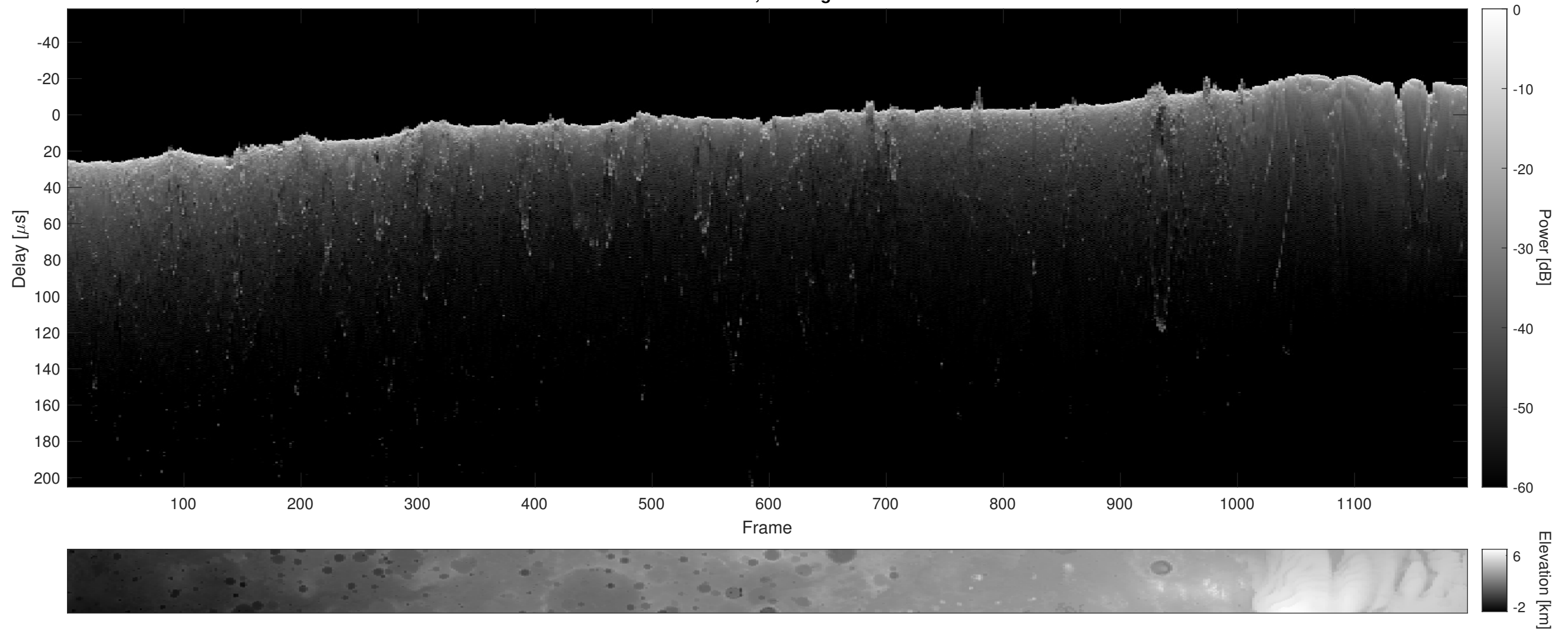
Orbit 6897, Cluttergram
