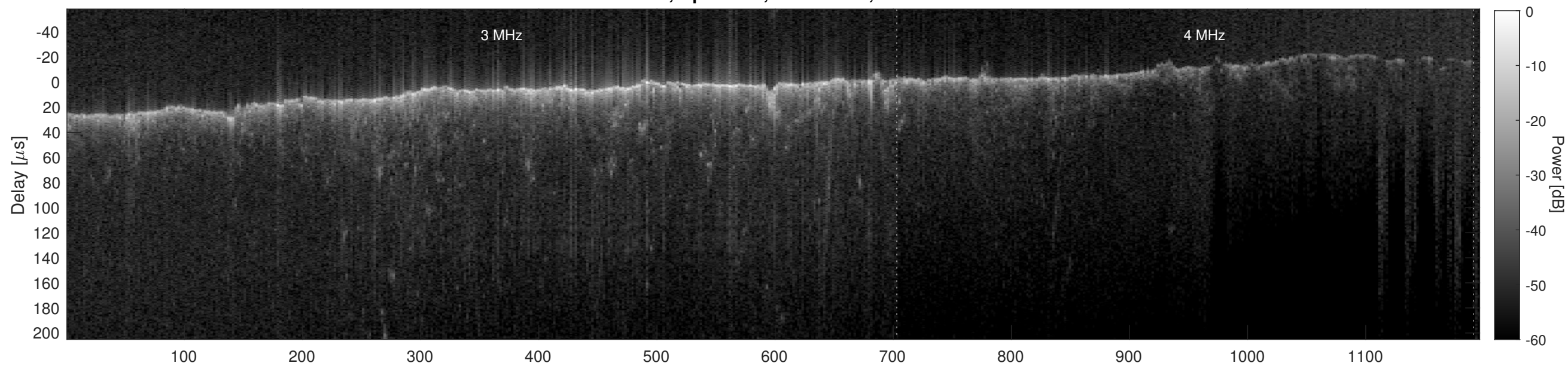
Orbit 6897, Cluttergram
