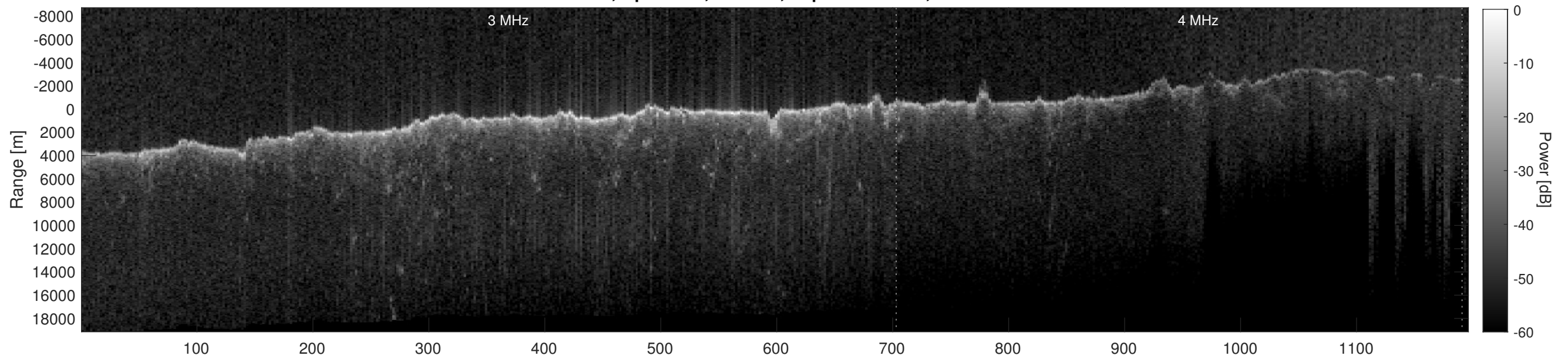
Orbit 6897, Depth-Corrected Cluttergram
