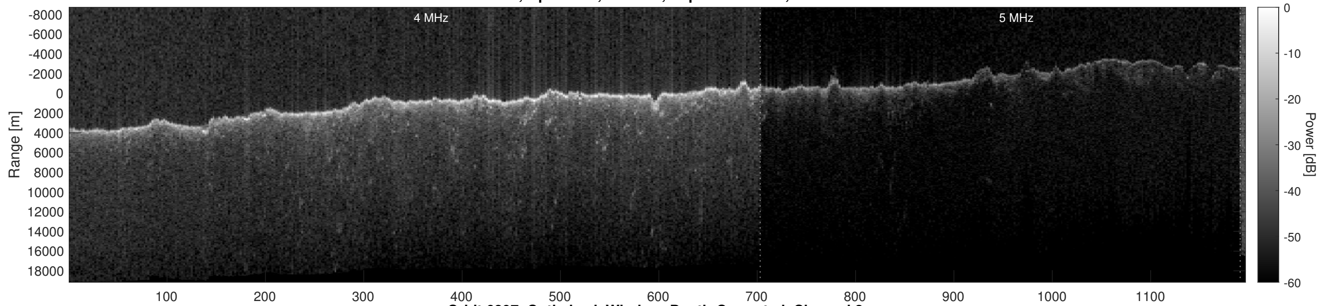
Orbit 6897, Optimized, Window, Depth-Corrected, Channel 2
