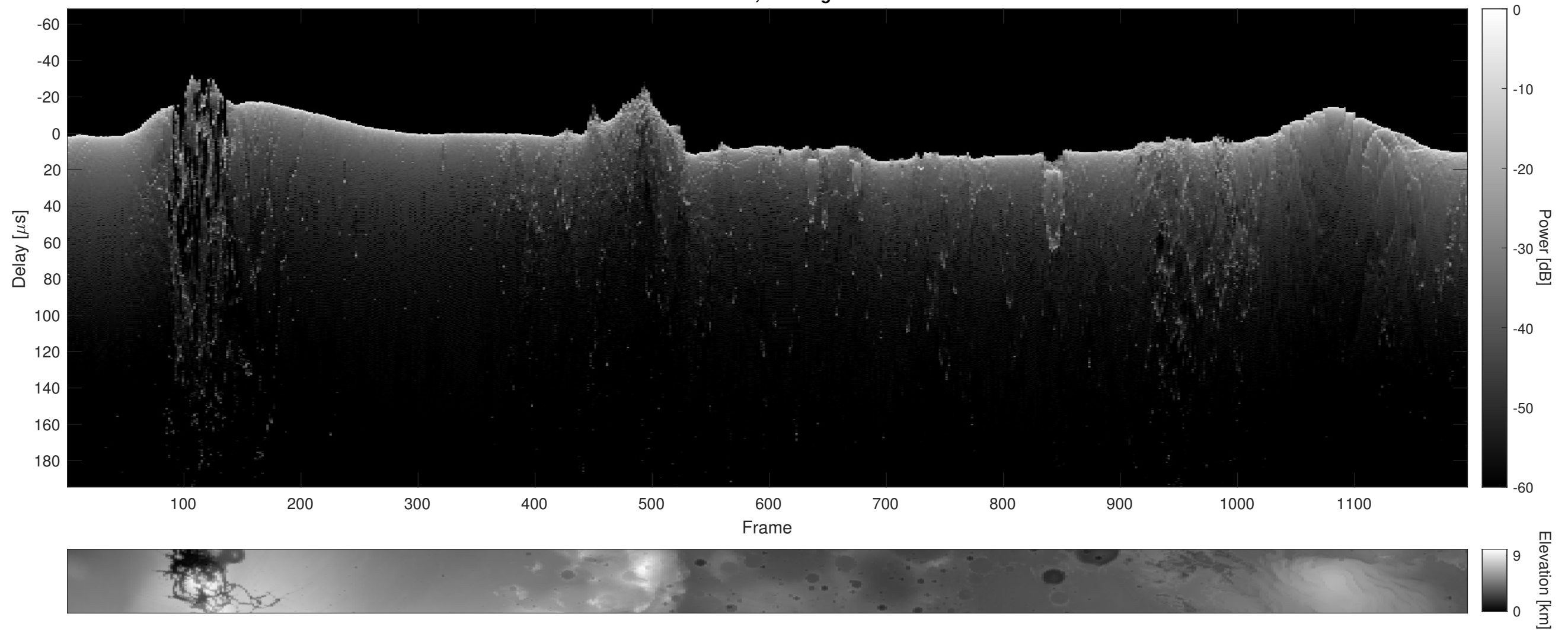
Orbit 6898, Cluttergram
