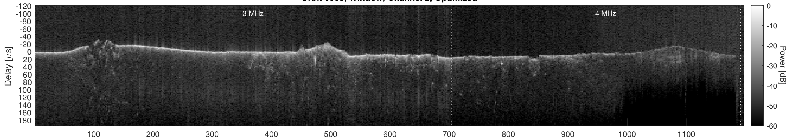
Orbit 6898, Cluttergram
