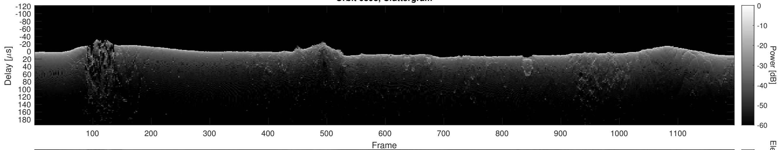
Orbit 6898, Cluttergram
