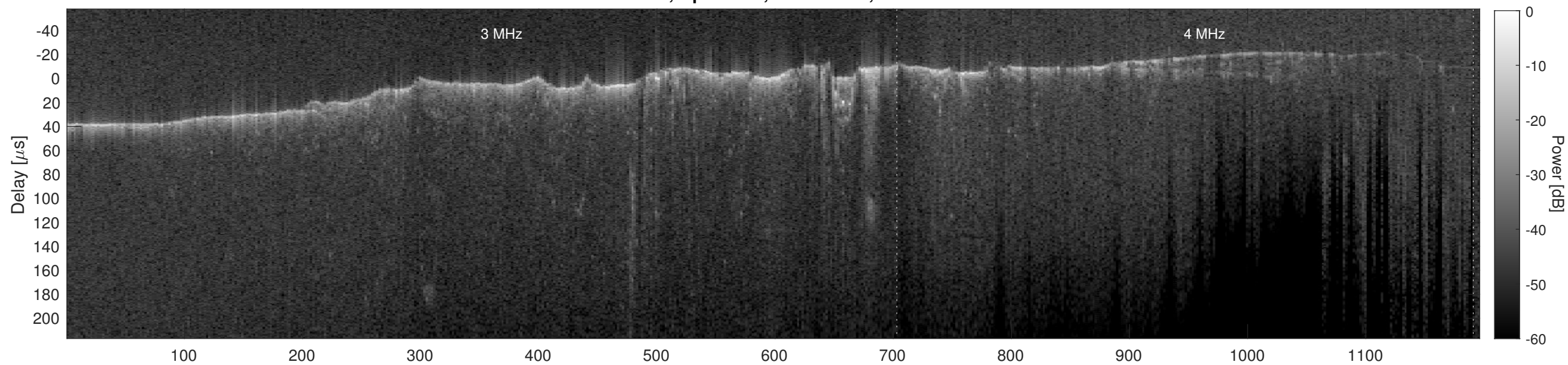
Orbit 6899, Cluttergram
