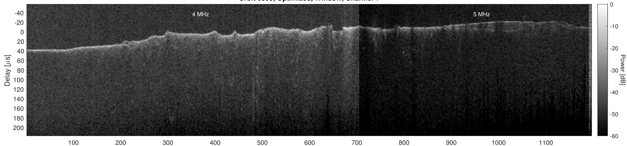
Orbit 6899, Optimized, Window, Channel 2
