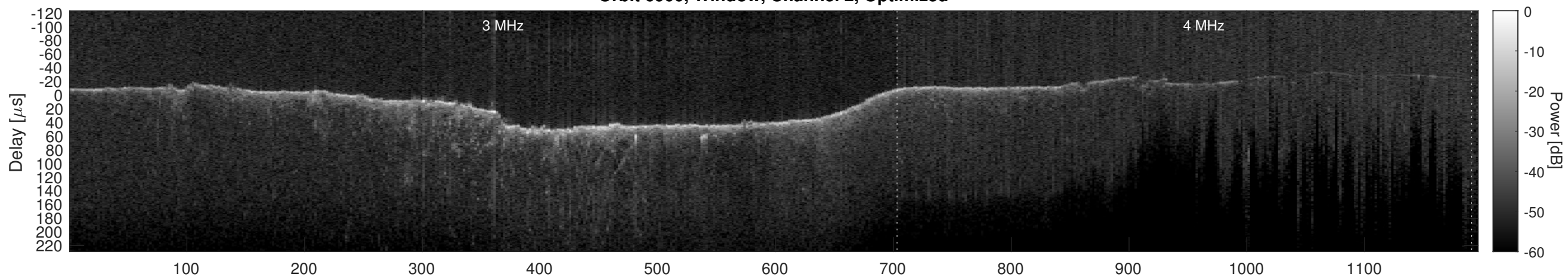
Orbit 6900, Cluttergram
