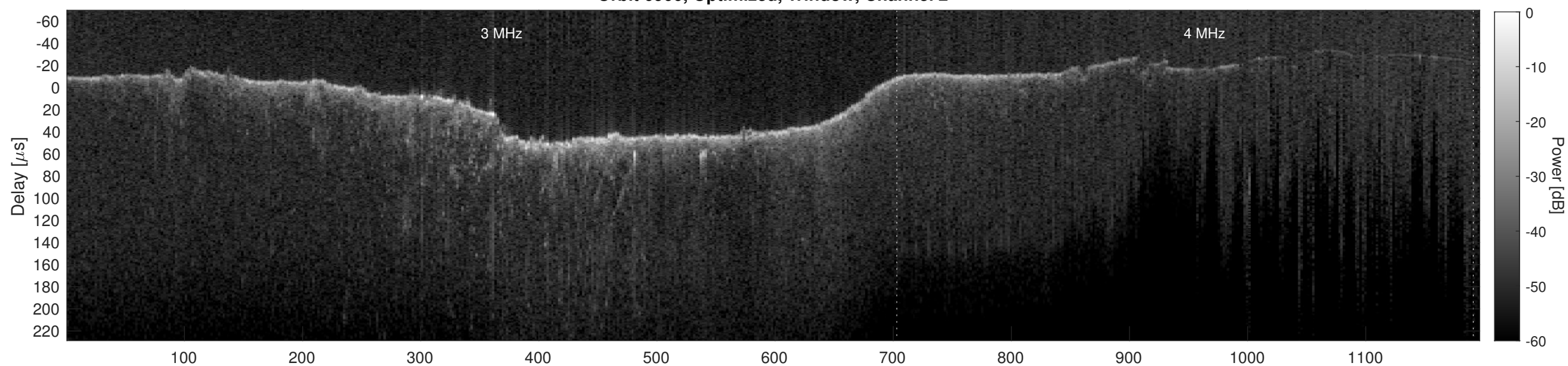
Orbit 6900, Cluttergram
