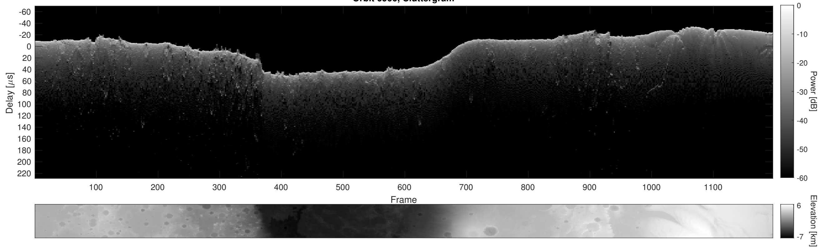
Orbit 6900, Cluttergram
