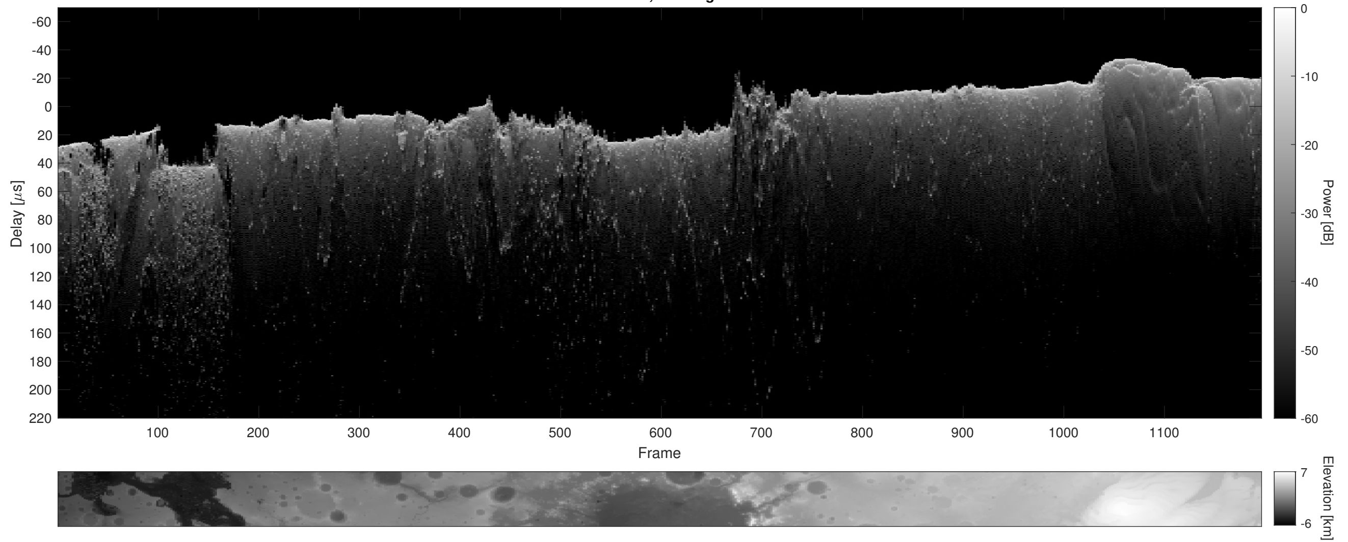
Orbit 6901, Cluttergram
