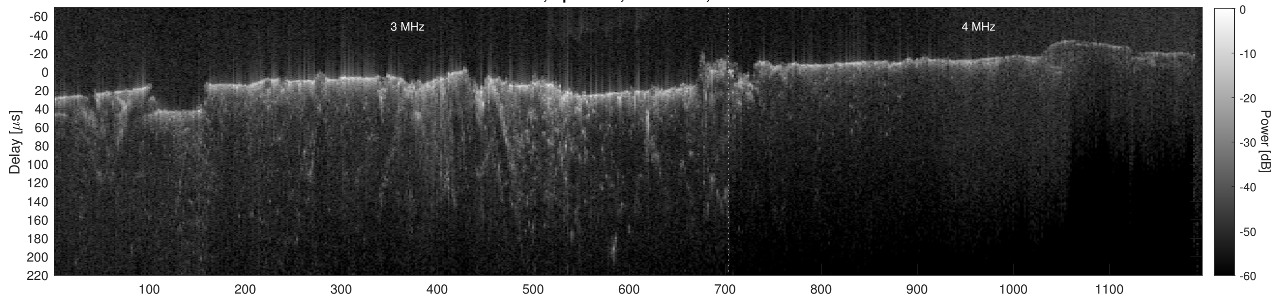
Orbit 6901, Cluttergram
