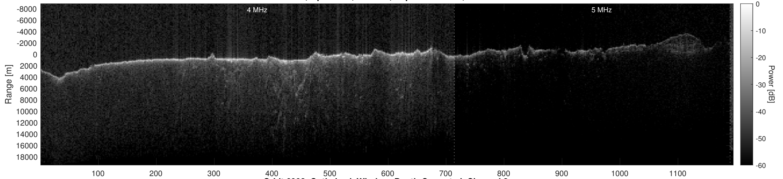
Orbit 6902, Optimized, Window, Depth-Corrected, Channel 2
