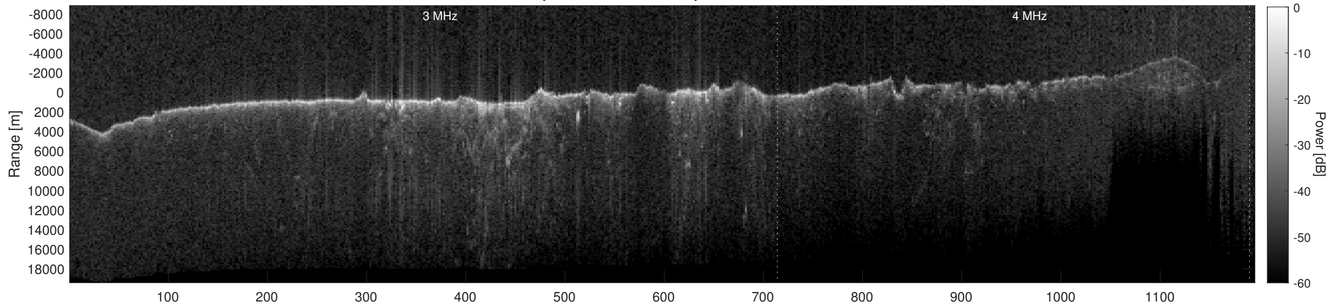
Orbit 6902, Depth-Corrected Cluttergram
