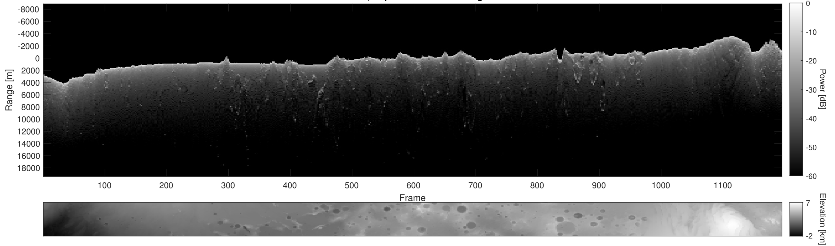
Orbit 6902, Depth-Corrected Cluttergram
