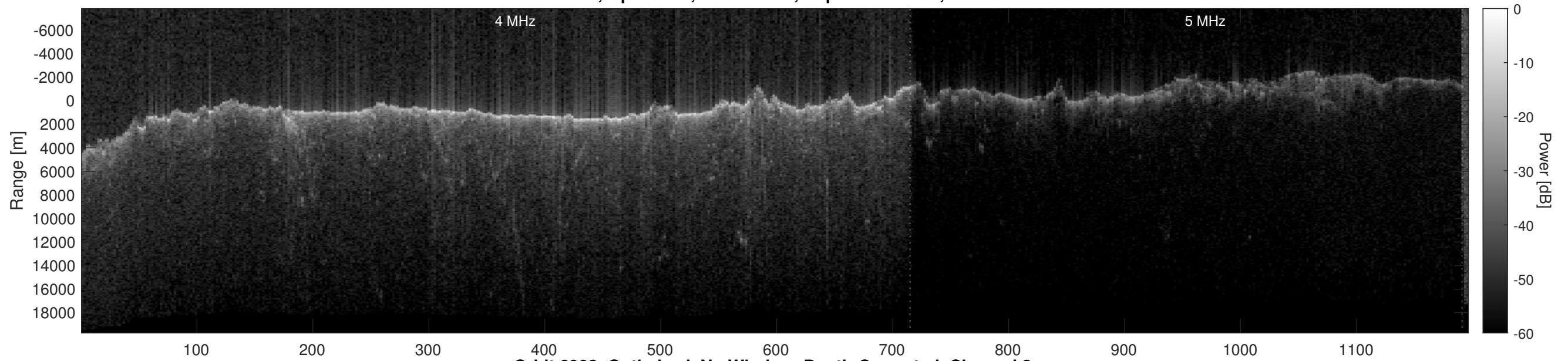
Orbit 6903, Optimized, No Window, Depth-Corrected, Channel 2
