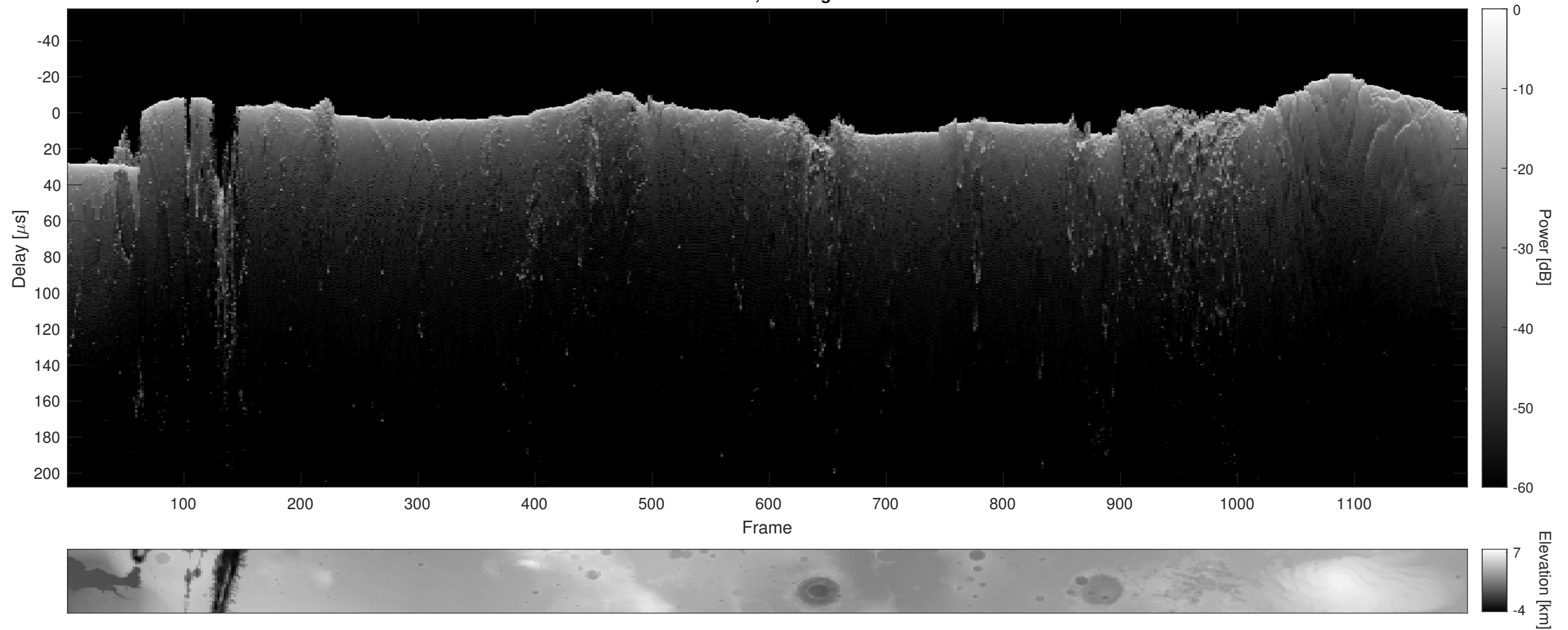
Orbit 6905, Cluttergram
