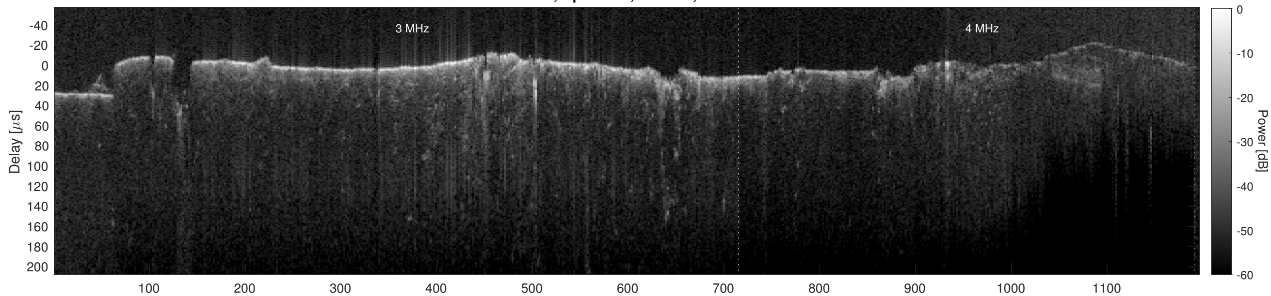
Orbit 6905, Cluttergram
